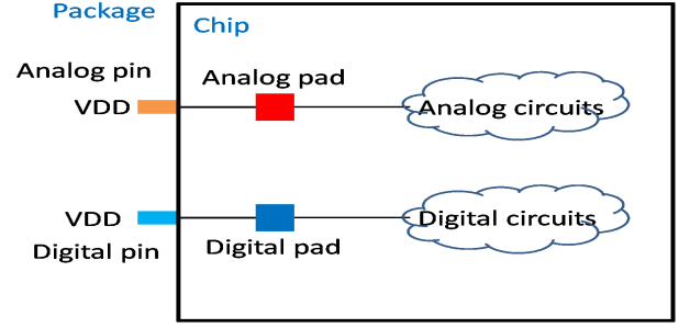
Fig. 10. Separation of digital and analog power/ground pads.
