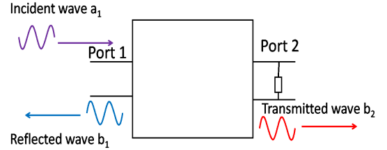
Fig. 5. Definition of S-parameter for a two-port system.
