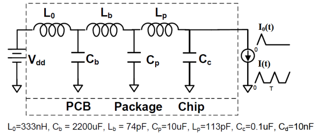
Fig. 2. Illustration of power delivery system.
