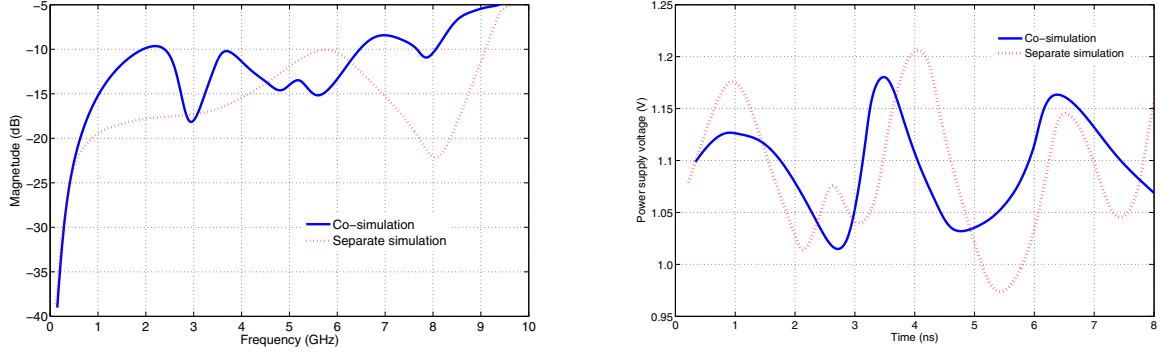
Fig. 8. Comparison of the S_{11} parameter and the power supply voltage from chip, package and board co-simulation and these from separate simulation.
