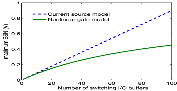
Fig. 6. Negative feedback effect for nonlinear gate models.
