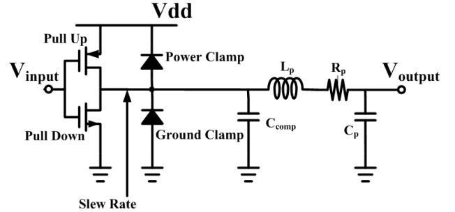
Fig. 7. IBIS model for I/O buffers.
