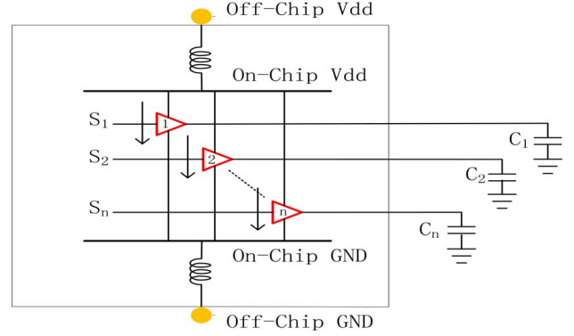
Fig. 1. SSN caused by the simultaneous switching of I/O buffers.
