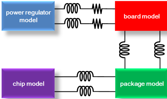
Fig. 4. Power delivery system modeling for SSN.
