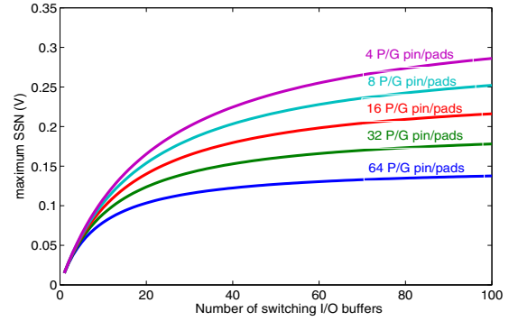
Fig. 11. Relationship between SSN and the number of switching I/O buffers for different number of power/ground pins/pads.
