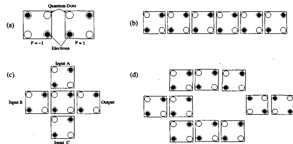
Fig. 1. (a) Shows the two polarization values for QCA cells. (b) A QCA wire. (c) A QCA majority gate, which is the fundamental logic gate implementing AB + BC + AC . (d) A QCA inverter.
