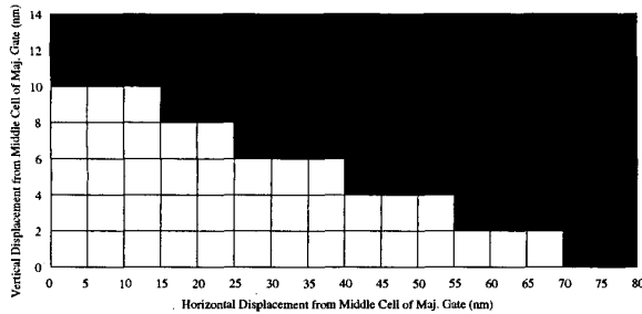
Fig. 3. A schmoop plot showing pass (white) vs. fail (black) for the horizontal and vertical displacements of the horizontal input to a majority gate, such as Input B in Fig. 1(c).
