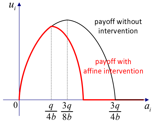
Fig. 6. Plot of u_i against a_i when the manager chooses the affine intervention rule (7) and the other user chooses a_i .
