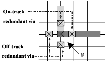
Fig. 8. Illustration of on- and off-track redundant vias.
