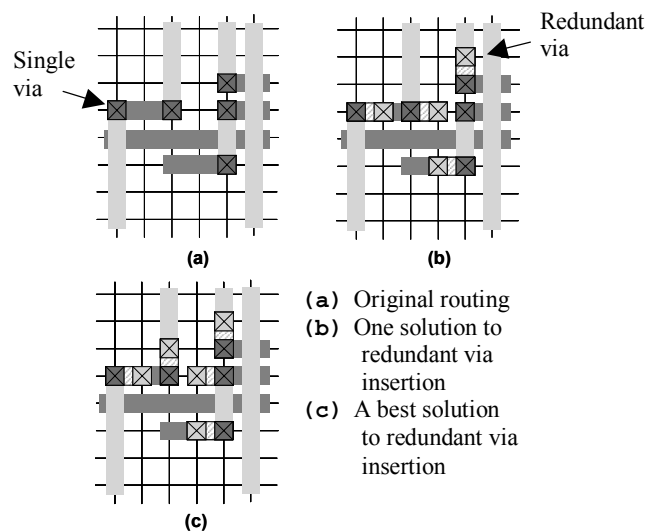
Fig. 1. Illustration of redundant via insertion.
