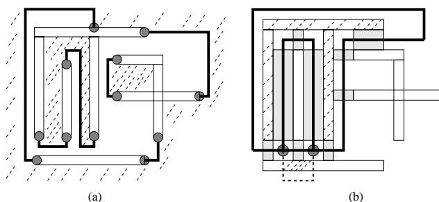
Figure 9: (a) Bright-field alternating PSM (positive resist) for a layout consisting of four features (eight rectangles). Crosshatched areas are 0 phase; other areas are 180 phase (features are defined by edges between 0- and 180-phase regions). Dark lines indicate phase edges (spurious features) that must be exposed away with a trim mask. (b) Dark-field alternating PSM (negative resist). “Routes” between 0- and 180-phase regions (features) must cover all separations that are less than B , i.e., phase conflicts. The solution for the feature at the bottom of the figure assumes a hypothetical partial-shifter (“vertex splitting”) approach to resolve the odd cycle in the conflict graph without changing feature placement.
