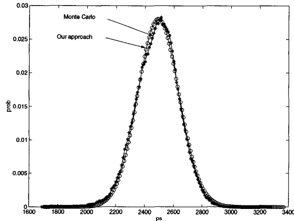
Figure 5. Comparison of Monte Carlo simulation and analytical approach for total delay variability
