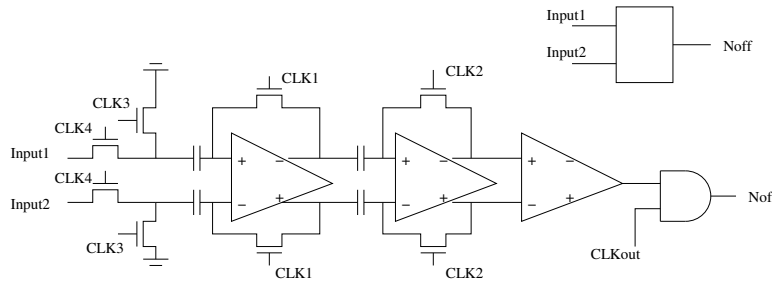
Figure 5: Current comparator.
