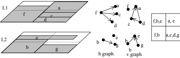
Figure 3 After a z-neighbor swap operation on b and f
