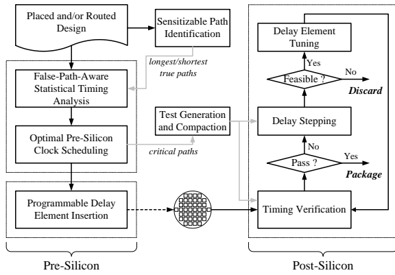
Fig. 1. The proposed clock scheduling methodology.
