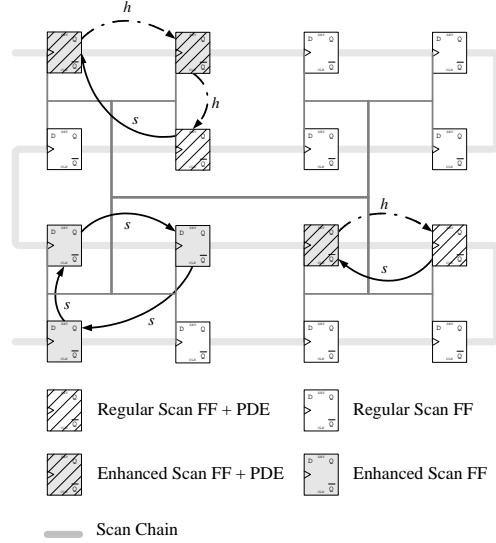
Fig. 8. The delay fault testing scheme for post-silicon clock scheduling.
