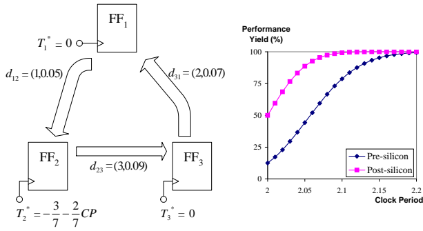
Fig. 3. (Left) a sequential circuit, and (right) timing yields of pre-silicon and post-silicon clock scheduling.
