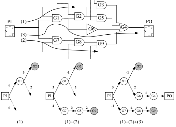
Fig. 2. Implicit enumeration of true paths using dynamic delay path tree.
