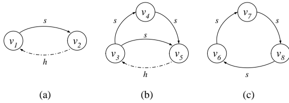
Fig. 5. The timing critical subgraph of \mathcal{G}^{CP} with 3 components.
