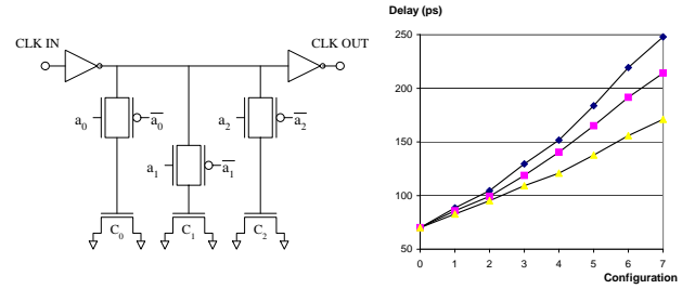
Fig. 4. A programmable delay element circuit and its delay curves for different delay ranges.
