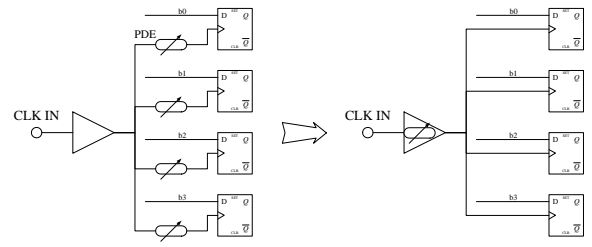
Fig. 6. Reducing number of programmable delay elements.
