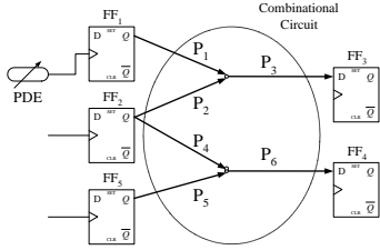
Fig. 7. Example of requirement on test diagnostic capability.
