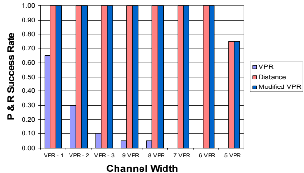
Figure 11. P&R success rate on routing-poor architectures
