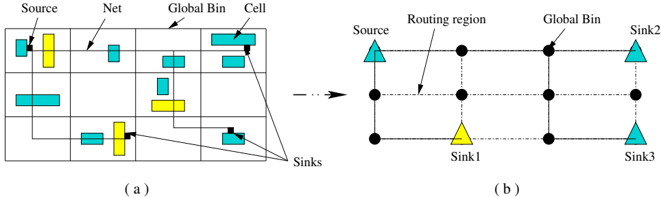
Fig. 1. (a) Layout. (b) The corresponding routing graph.
