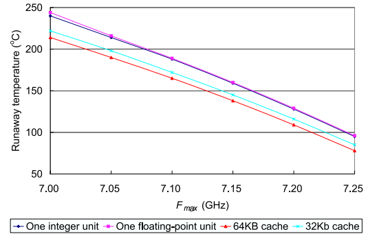
Fig. 6. Runaway temperatures.
