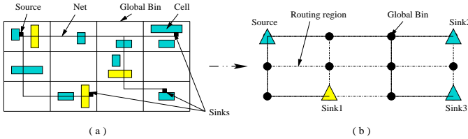
Fig. 1. (a) Layout. (b) The corresponding routing graph.
