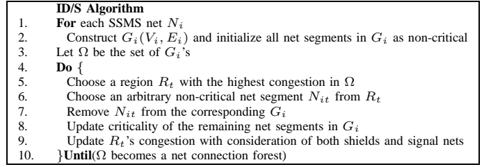
Fig. 4. Phase I algorithm: Global routing synthesis based on iterative deletion. When shields are considered in line 9, it is ID/S, otherwise, it is ID.
