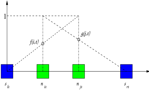
Fig. 2. Illustration of K_{it,jt} computation in a given block.
