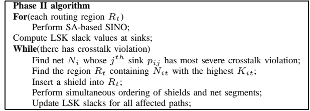
Fig. 7. Phase II algorithm.
